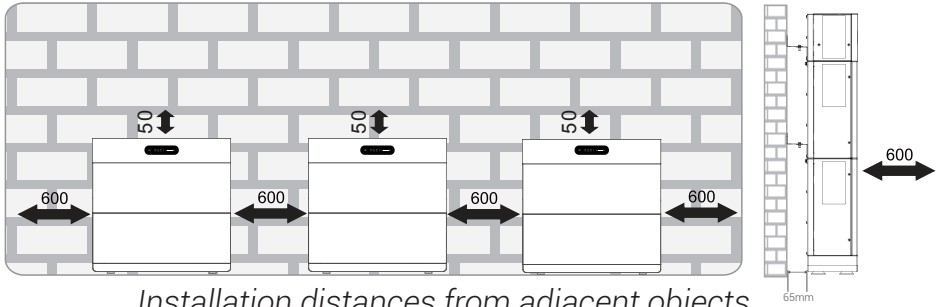
Installation distances from adjacent objects
